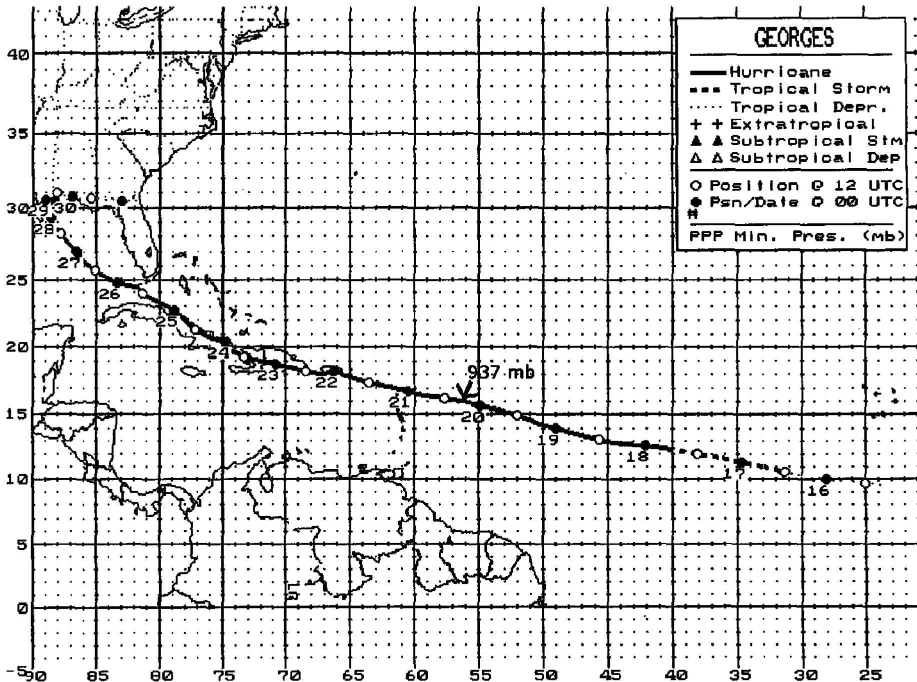
Best Track for Hurricane Georges, 15 September - 1 October, 1998.
