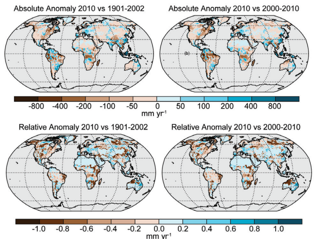
FIG. 2.26. Absolute and relative anomalies for river discharge in 2010 with respect to the long-term average over the 20th century and for the last decade.
