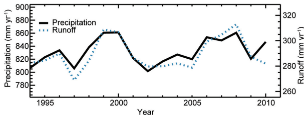
FIG. 2.24. Annual continental precipitation from GPCC full product extended with the monitoring product for 2010 and the corresponding water balance model-simulated continental runoff using NCEP air temperature forcing.
