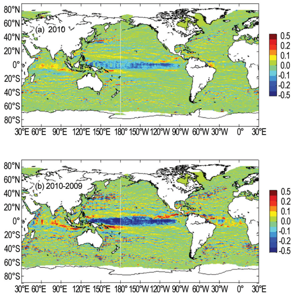
FIG. 3.19. Global zonal geostrophic anomalies for 2010 (top) and 2010 minus 2009 (bottom), cm s -1 , derived from a synthesis of drifters, altimetry, and winds.
