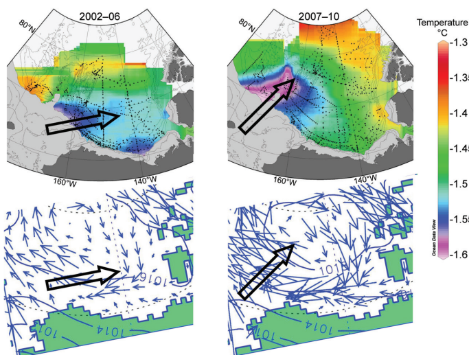
FIG. 5.9. Top panels: potential temperature (°C) in the Canada Basin at the S = 33.1 isohaline. Bottom panels: sea level atmospheric pressure (hPa) and simulated wind-driven component of ice drift. Left and right panels: 2002–06 and 2007–10, respectively. Large arrows show suggested spreading of Pacific winter waters.
