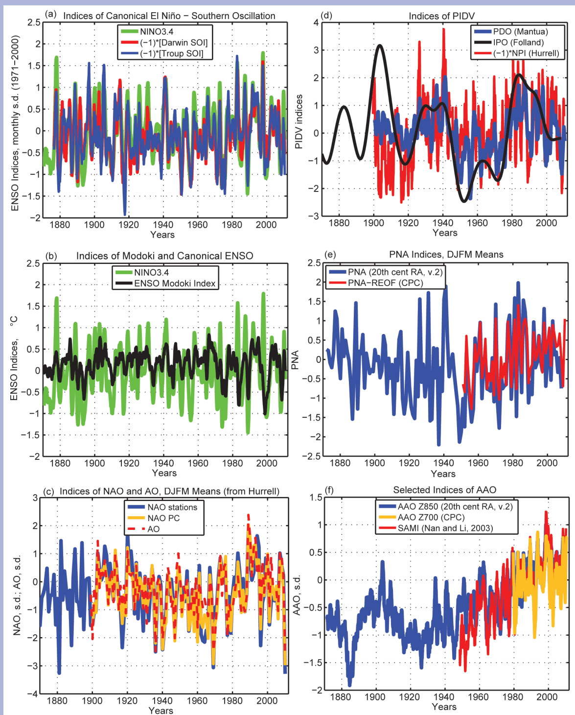
FIG. I.3. Selected indices of climate variability, as specified in Table 2.3, for the period 1880–2010, grouped into categories: (a) Canonical El Niño – Southern Oscillation (ENSO); (b) the Modoki variant of ENSO; (c) Northern Hemisphere oscillations (NAO, AO, NAM) for the boreal cold season; (d) indices of Pacific Inter-decadal Variability; (e) Pacific-North American indices for the boreal cold season; (f) Southern
