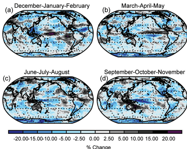
FIG. 2.22. Seasonal global cloudiness anomalies determined using the PATMOS-X dataset for (a) Dec 2009–Feb 2010, (b) Mar–May 2010, (c) Jun–Aug 2010, and (d) Sep–Nov 2010. Seasonal anomalies are calculated by subtracting the mean cloud fraction over the 1982–2010 base period from that of 2010.
