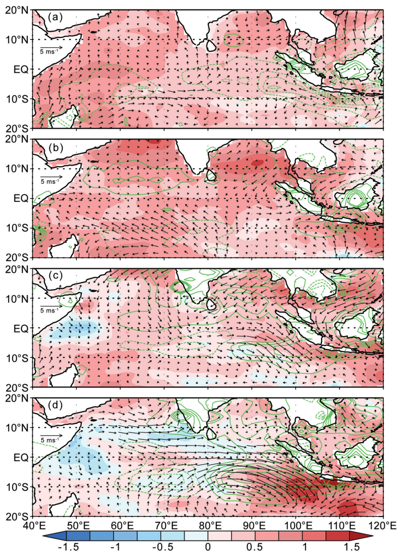
FIG.4.38. Sea surface temperature ( ^{\circ}\text{C} , colored scale), precipitation (green contour: \pm 1 , \pm 2 , ..., \pm 5 \text{ mm day}^{-1} ), and surface wind anomalies during (a) December–February 2009/10; (b) March–May 2010; (c) June–August 2010; and (d) September–November 2010. Anomalies were calculated relative to the climatology over the period 1982–2009. These are based on the NCEP optimum interpolation SST (Reynolds and Chelton 2010), monthly GPCP precipitation analysis ( http://precip.gsfc.nasa.gov/ ), and JRA-25 atmospheric reanalysis (Onogi et al. 2007).
