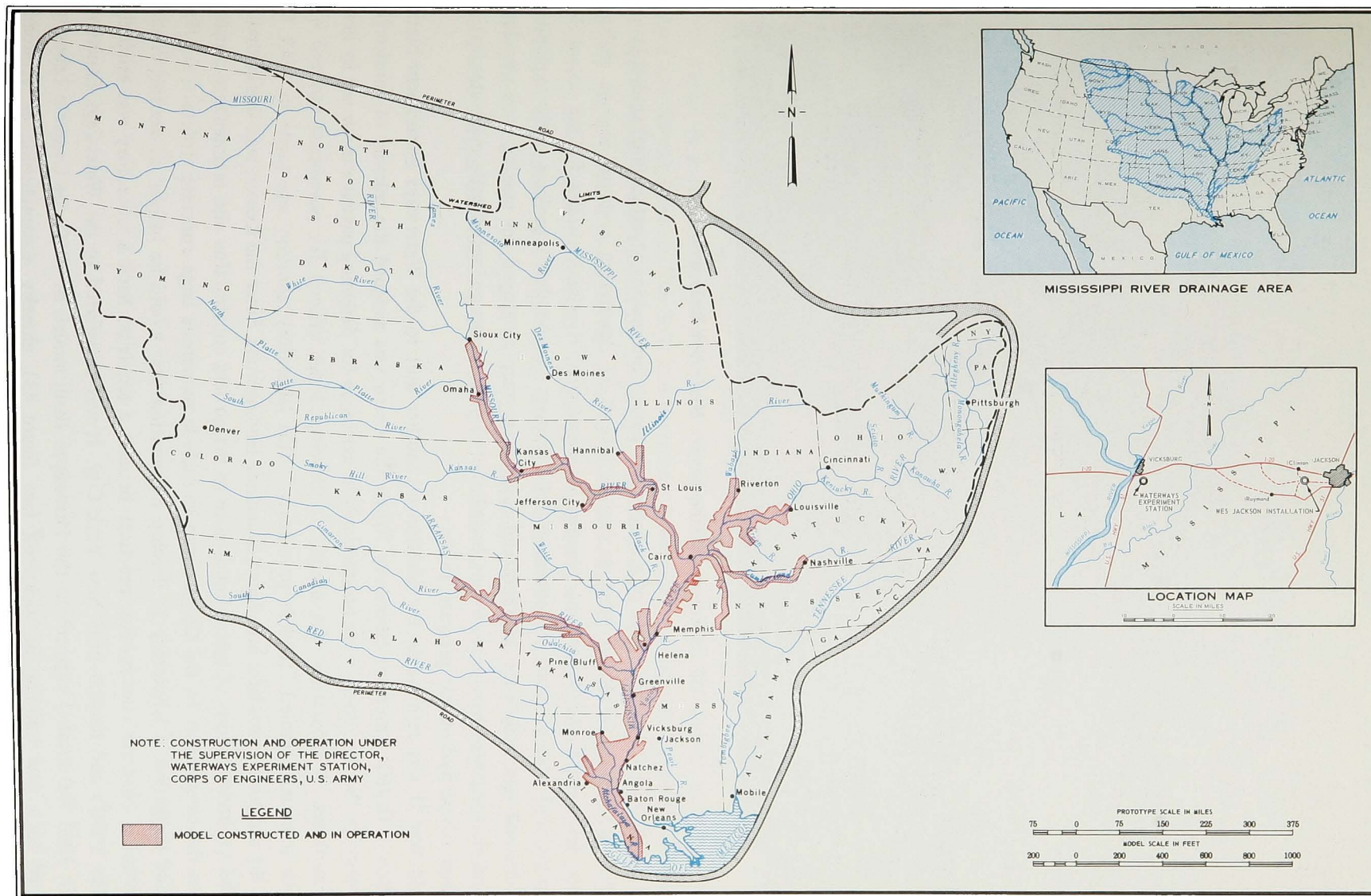
Figure 41. Prototype area reproduced in comprehensive Mississippi Basin model
