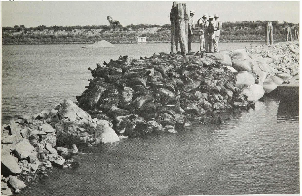
Figure 67. Experimental section of sand-filled nylon bags for dike construction
