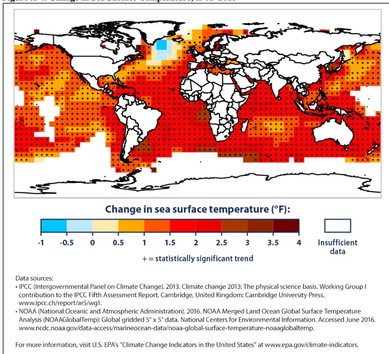
Figure A-4. Change in Sea Surface Temperature, 1901–2015
