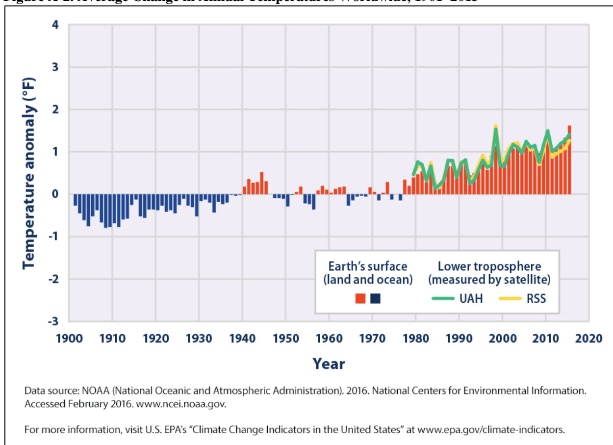
Figure A-2. Average Change in Annual Temperatures Worldwide, 1901–2015
