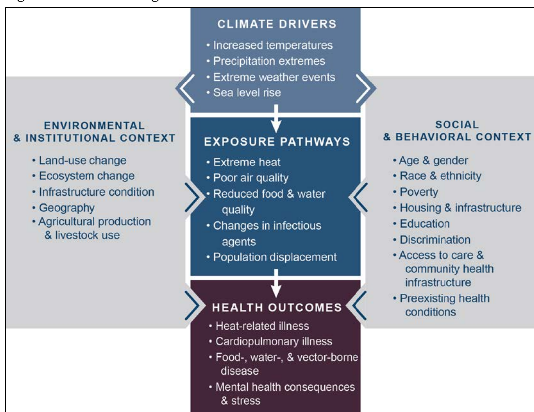
Figure 3. Climate Change and Human Health
