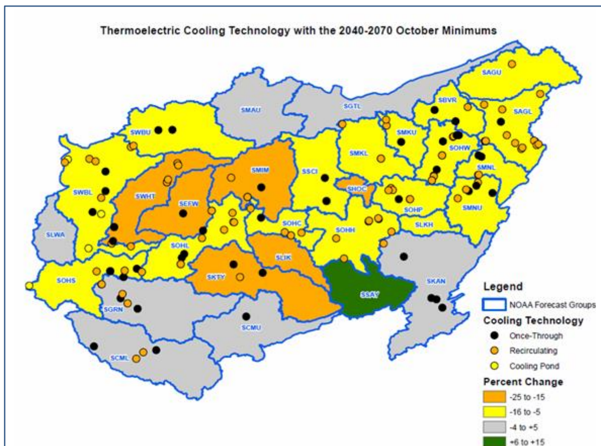
Figure 10-6: Thermoelectric Power Plants Shown by Cooling Technology
