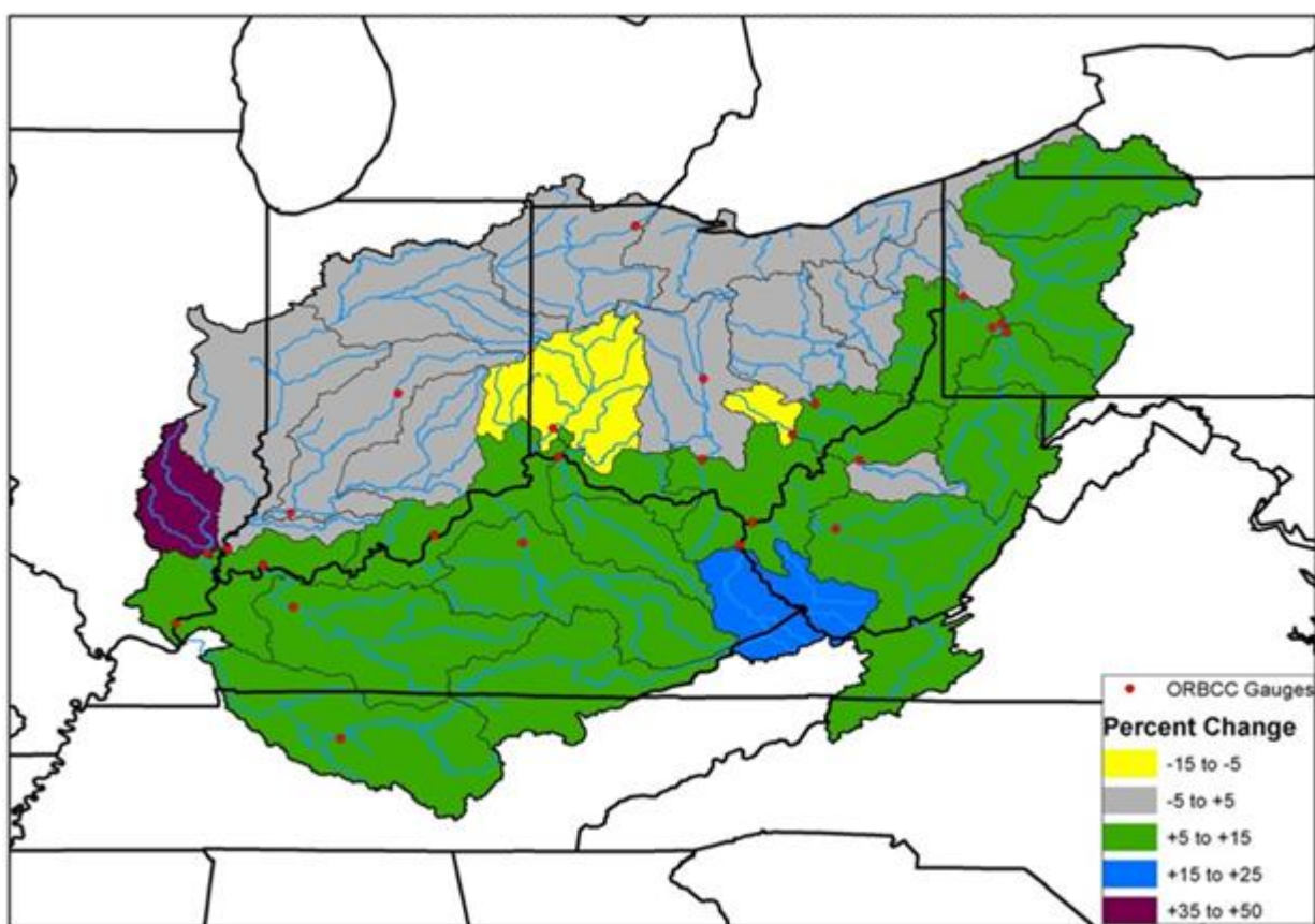
Figure A.8-F1: October Minimum Streamflow
