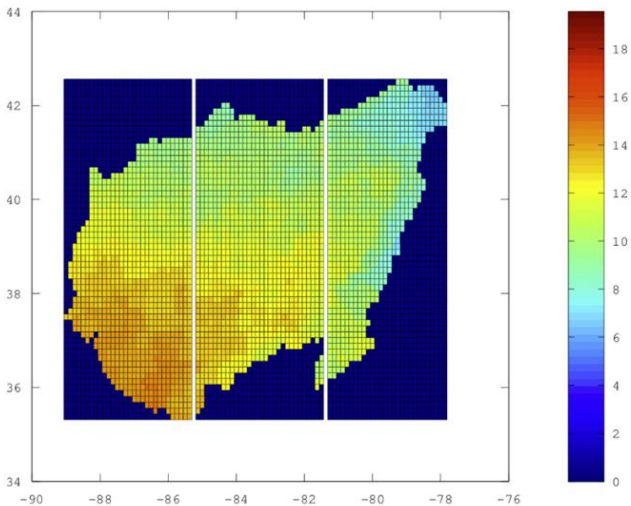
Figure A-16: Graphic Display of Precipitation Base Model Results (1950–2000)–IWR
