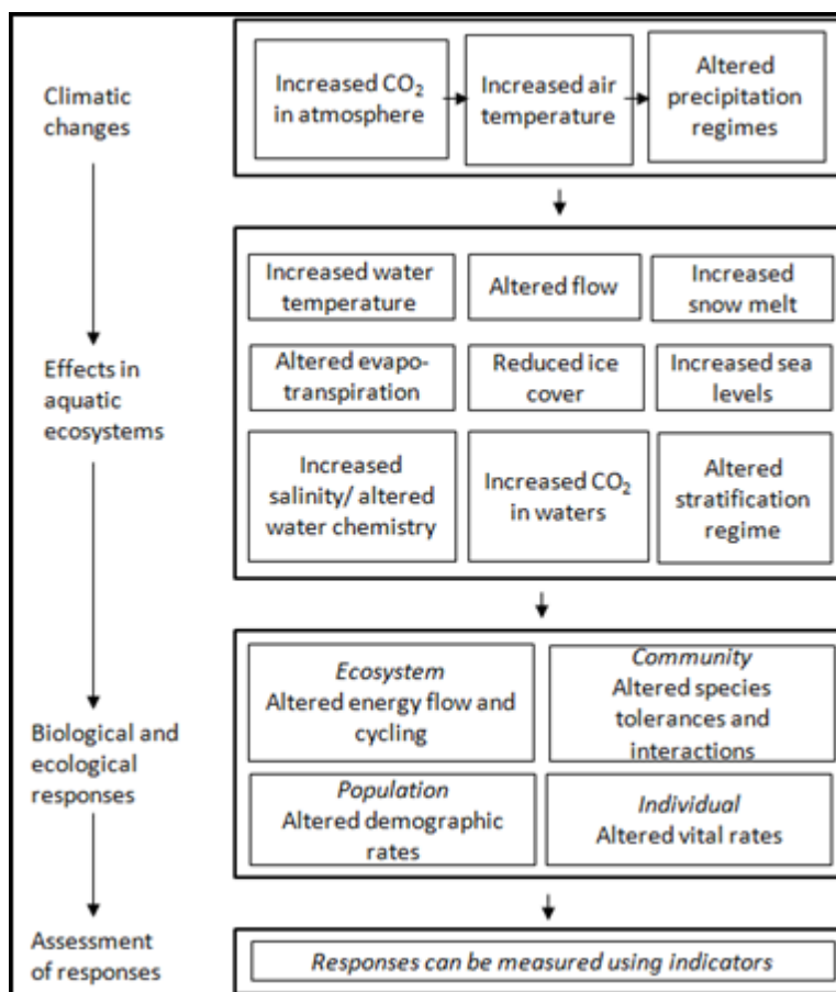
Figure 8-1: Conceptual Diagram of CC Effects on Aquatic Ecosystems and Possible Ecosystem Responses that Can Be Measured Using Biological or Ecological Indicators 7
