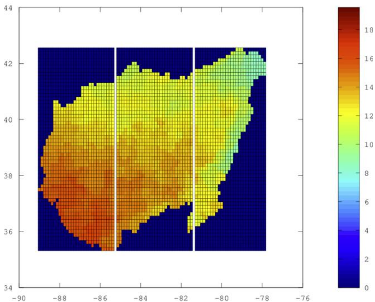
Figure A-12: Graphic Display of 2011–2040 Temperature Model Results (IWR)
