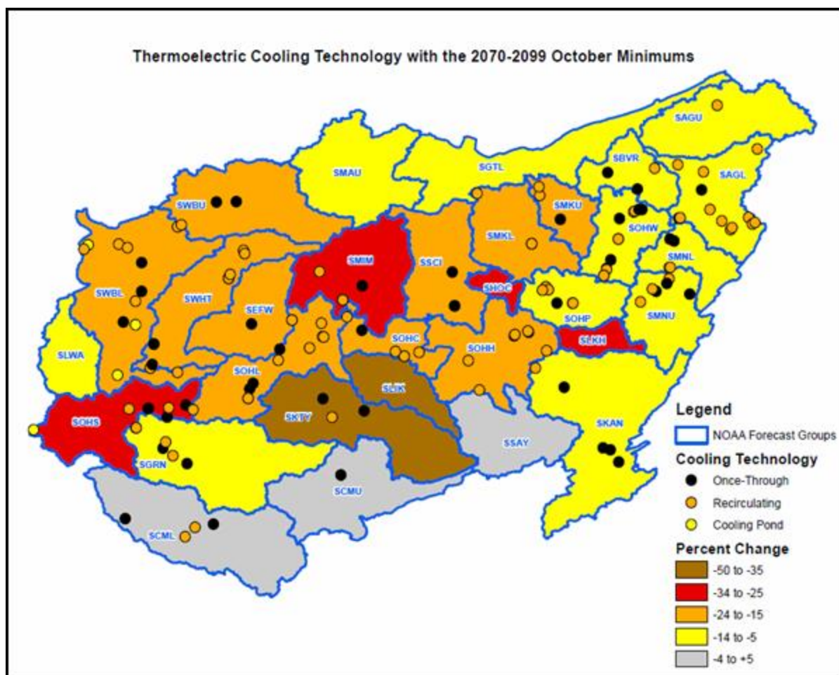
Figure 8-15: Thermoelectric Power Plants Extracting Surface Water for Cooling
