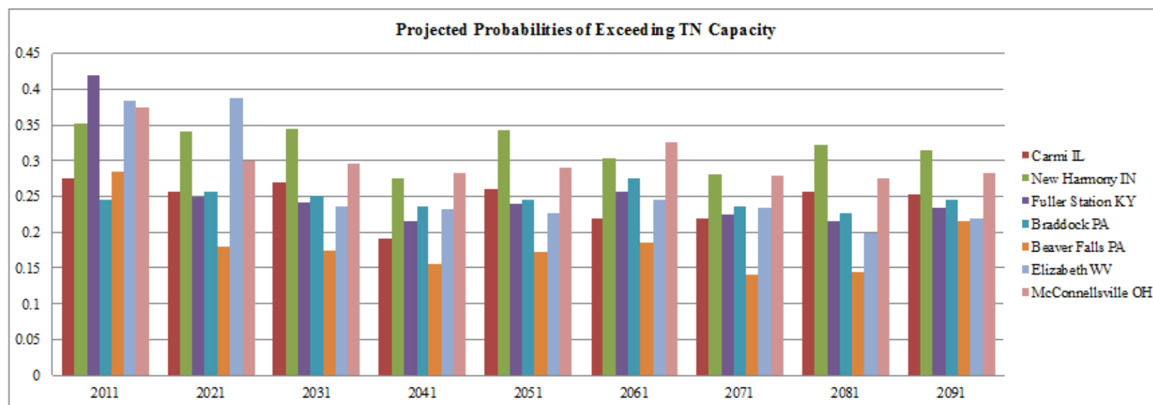
Figure B-7: Projected Probabilities of Exceeding TN Capacity
