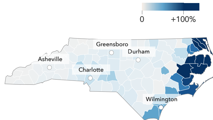
Change in total annual loss from 2021 to 2051
