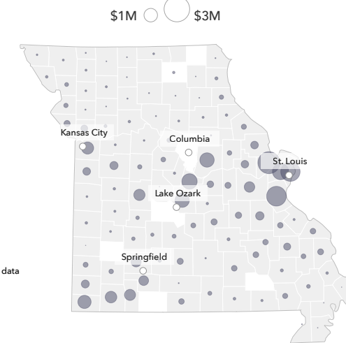
Total annual loss per county, 2021
