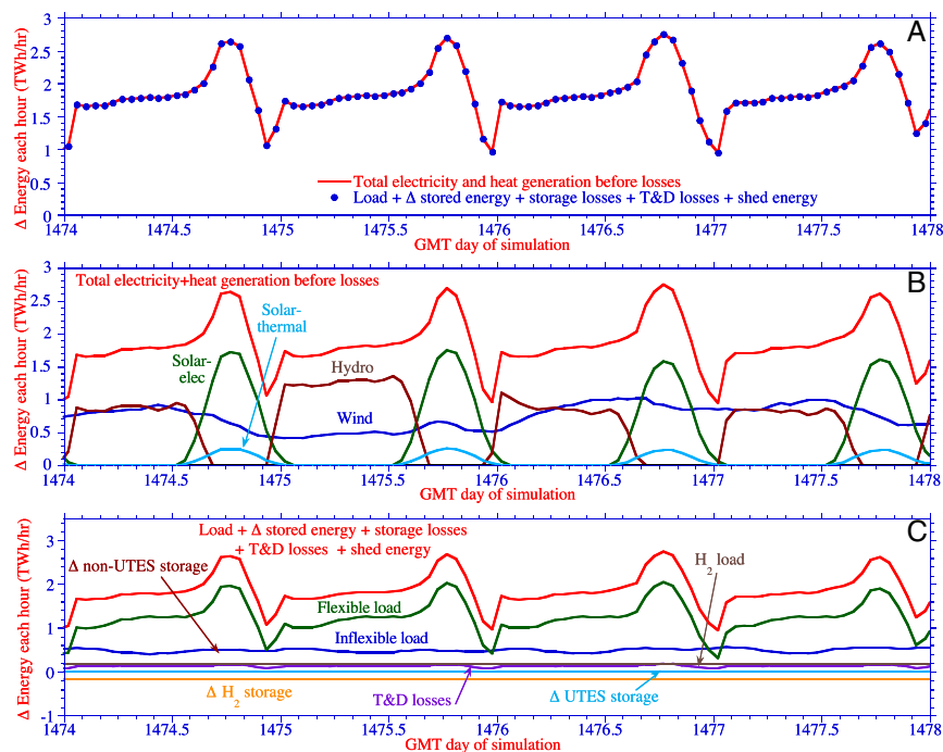
Fig. 4. (A) Time series comparison each hour of modeled CONUS-aggregated power generation vs. load plus losses plus changes in storage plus shedding for January 14–17, 2055. (B) Breakdown of power generation for the same period. (C) Breakdown of load plus losses plus changes in storage plus shedding.
