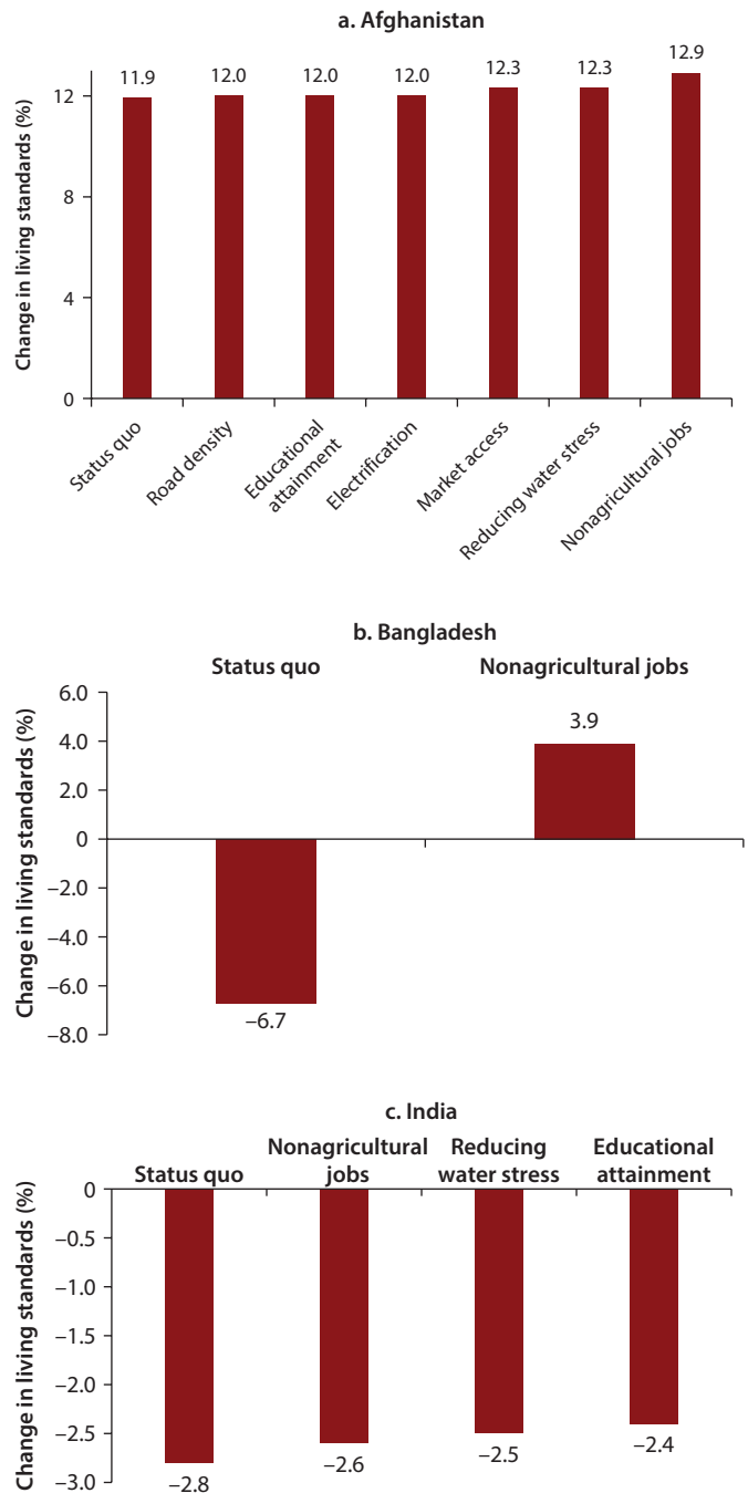
FIGURE 5.1 Good Development Outcomes Reduce Hotspots (Effects of Various Interventions on Living Standards in South Asia under the Carbon-Intensive Scenario, by 2050)
