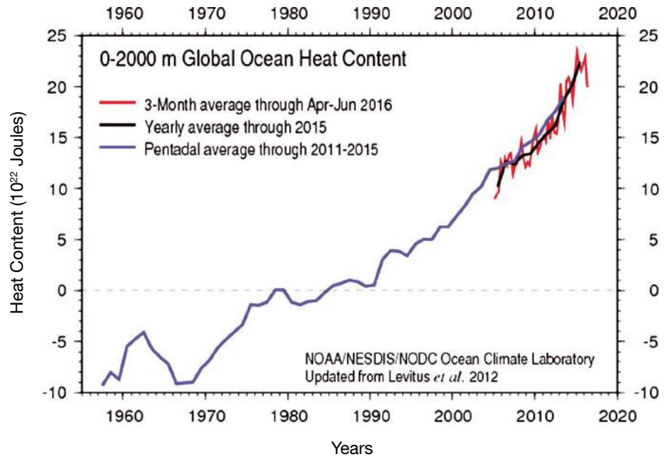
Figure 1.12 Plot of Global OHC 0-2000m as a pentadal trend from 1955-1959 to 2011-2015, with superimposed a yearly average from 2005-2015 and a three month average from January to March 2005 to April to June 2016; all averaged from 26 standard depths. From: https://www.nodc.noaa.gov/OC5/3M_HEAT_CONTENT/ Downloaded on 25 June 2016.
