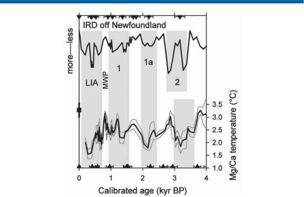
FIGURE 5-4 Variation of bottom temperature on the Labrador current inferred from Mg/Ca ratios in forams and the relation to the measure of ice-rafted debris (IRD) showing variations in North Atlantic temperature changes as reflected in deep-sea sediments. SOURCE: Marchitto and deMenocal (2003). Reproduced by permission of American Geophysical Union; copyright 2003.
