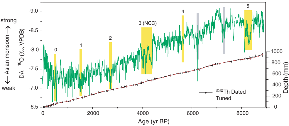
FIGURE 5-8 \delta^{18}\text{O} over the Holocene derived from a cave in eastern Asia. The yellow numbered bands correspond to times of ice-rafted debris in the North Atlantic shown in Figure 5-6 (Bond et al. 2001). SOURCE: Wang et al. (2005b). Reprinted with permission from AAAS; copyright 2005.
