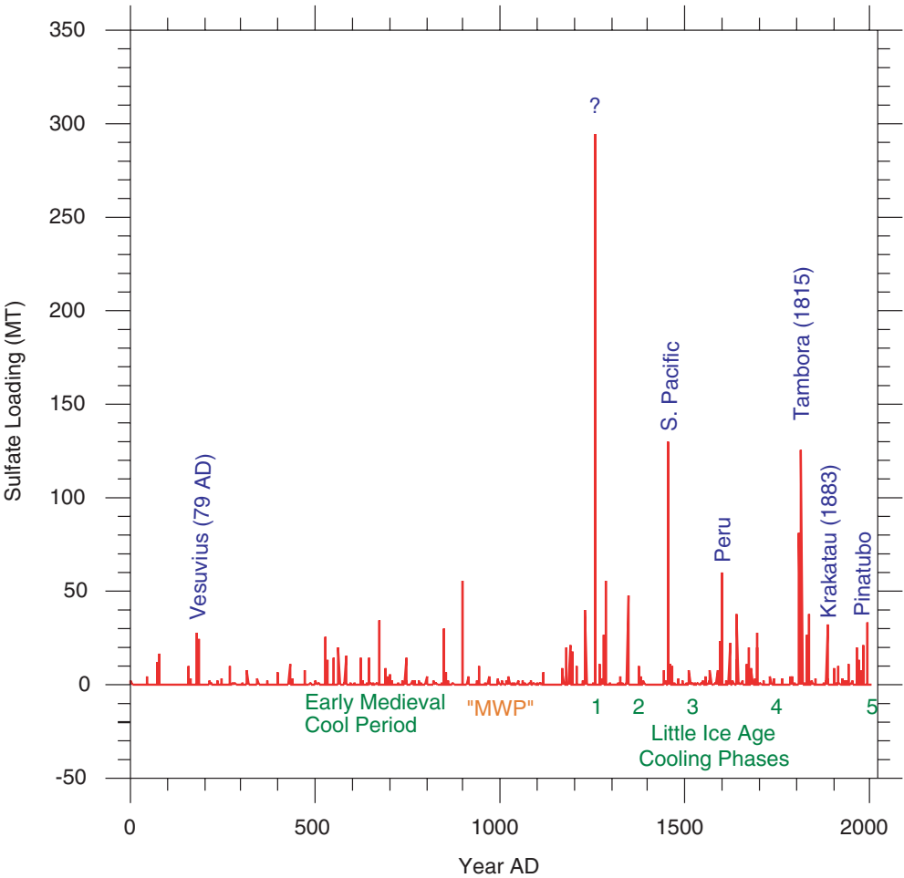
FIGURE 10-3 Ice core estimates of global stratospheric sulfate loading from volcanoes (A.D. 1–2005). SOURCE: T. Crowley, Duke University, 2006, unpublished material. Reprinted with permission; copyright 2006.
