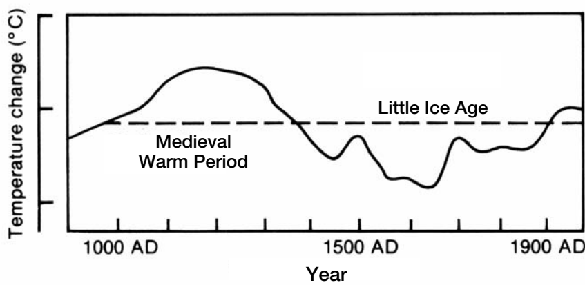
FIGURE O-3 Schematic description of global temperature variations in degrees Celsius for the last 1,100 years published more than 15 years ago. SOURCE: IPCC (1990). Reprinted with permission; copyright 1990, IPCC.
