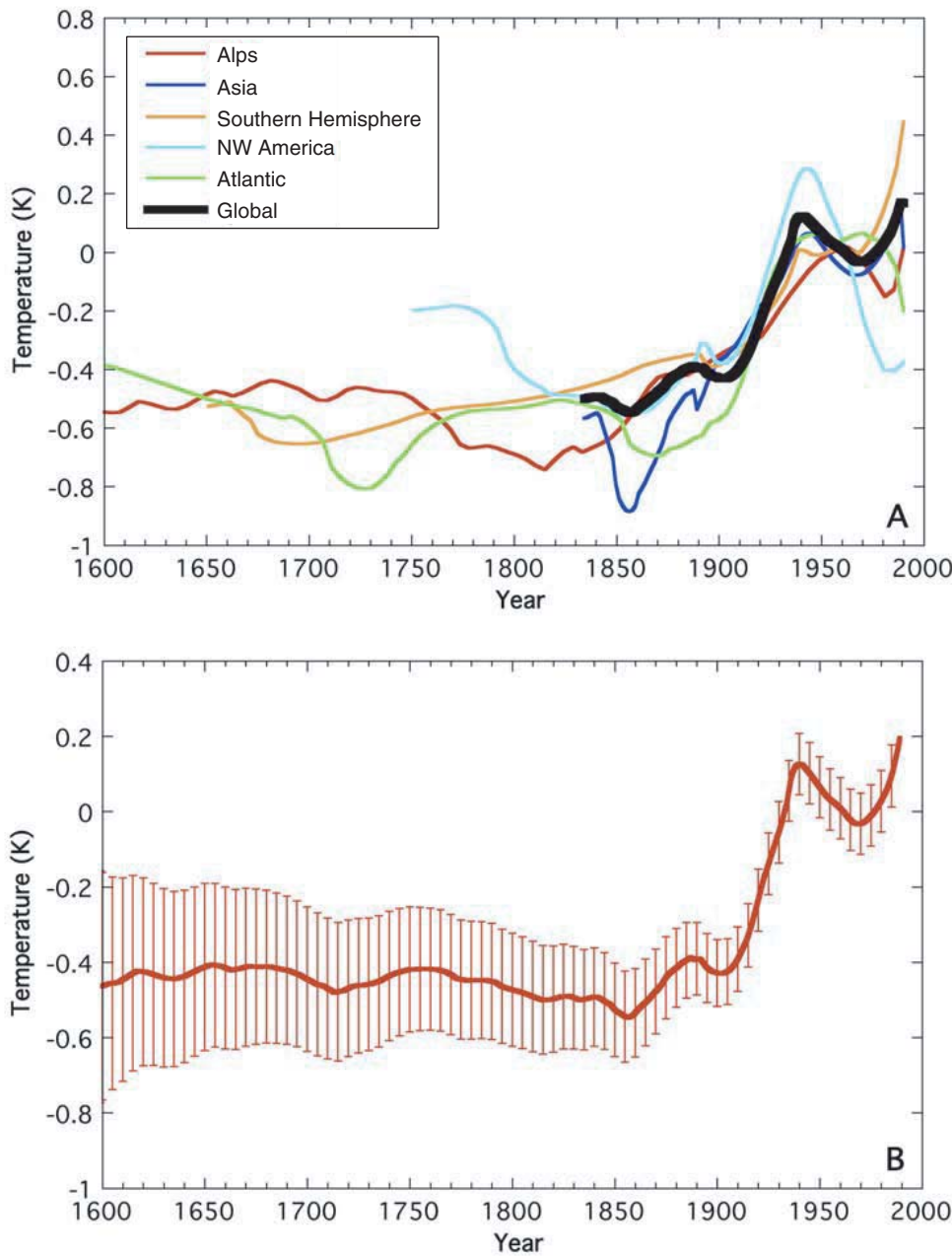
FIGURE 7-1 (A) Glacier-length-based temperature reconstruction for various regions. The black curve shows an estimated global mean value, obtained by giving weights of 0.5 to the Southern Hemisphere, 0.1 to Northwest America, 0.15 to the Atlantic sector, 0.1 to the Alps, and 0.15 to Asia. (B) Best estimate of the global mean temperature, obtained by combining the weighted global mean temperature for 1834–1990 with the average of temperature records at earlier times. The band indicates the estimated standard deviation. SOURCE: Oerlemans (2005a). Reprinted with permission from AAAS; copyright 2005.
