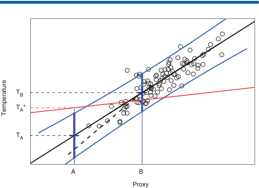
FIGURE 9-1 An illustration of using linear regression to predict temperature from proxy values. Plotted are 100 pairs of points corresponding to a hypothetical dataset of proxy observations and temperature measurements. The solid black line is the least-squares fitted line and the blue lines indicate 95 percent prediction intervals for temperature using this linear relationship. The dashed line and the red line indicate possible departures from a linear relationship between the proxy data and the temperature data. The figure also illustrates predictions made at proxy values A and B and the corresponding prediction intervals (wide blue lines) for the temperature.
