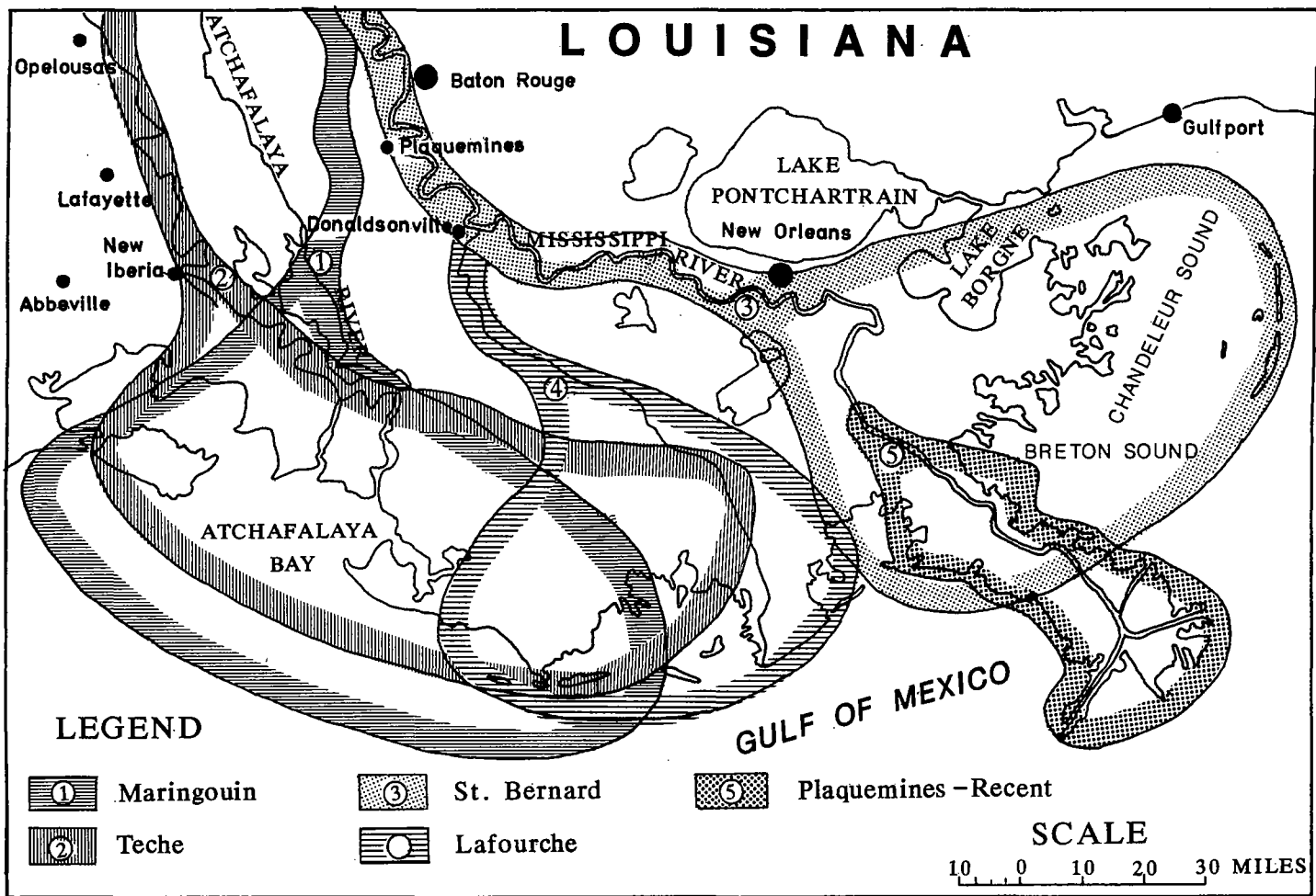
Figure 1. Delta complexes comprising the Mississippi River deltaic plain (from Kolb and Van Lopik 1966)
