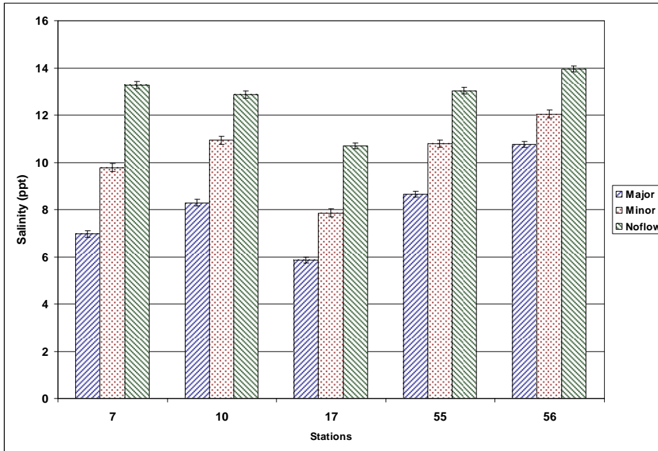
Figure 4. BA-04 mean ( \pm SE) salinity for the period 1999-2003 for 3 operational categories at YSI continuous recorder stations (major discharge >1,072 \text{ ft}^3\text{s}^{-1} ; minor discharge > 0 <1,072 \text{ ft}^3\text{s}^{-1} ; no flow =0 \text{ ft}^3\text{s}^{-1} ).
