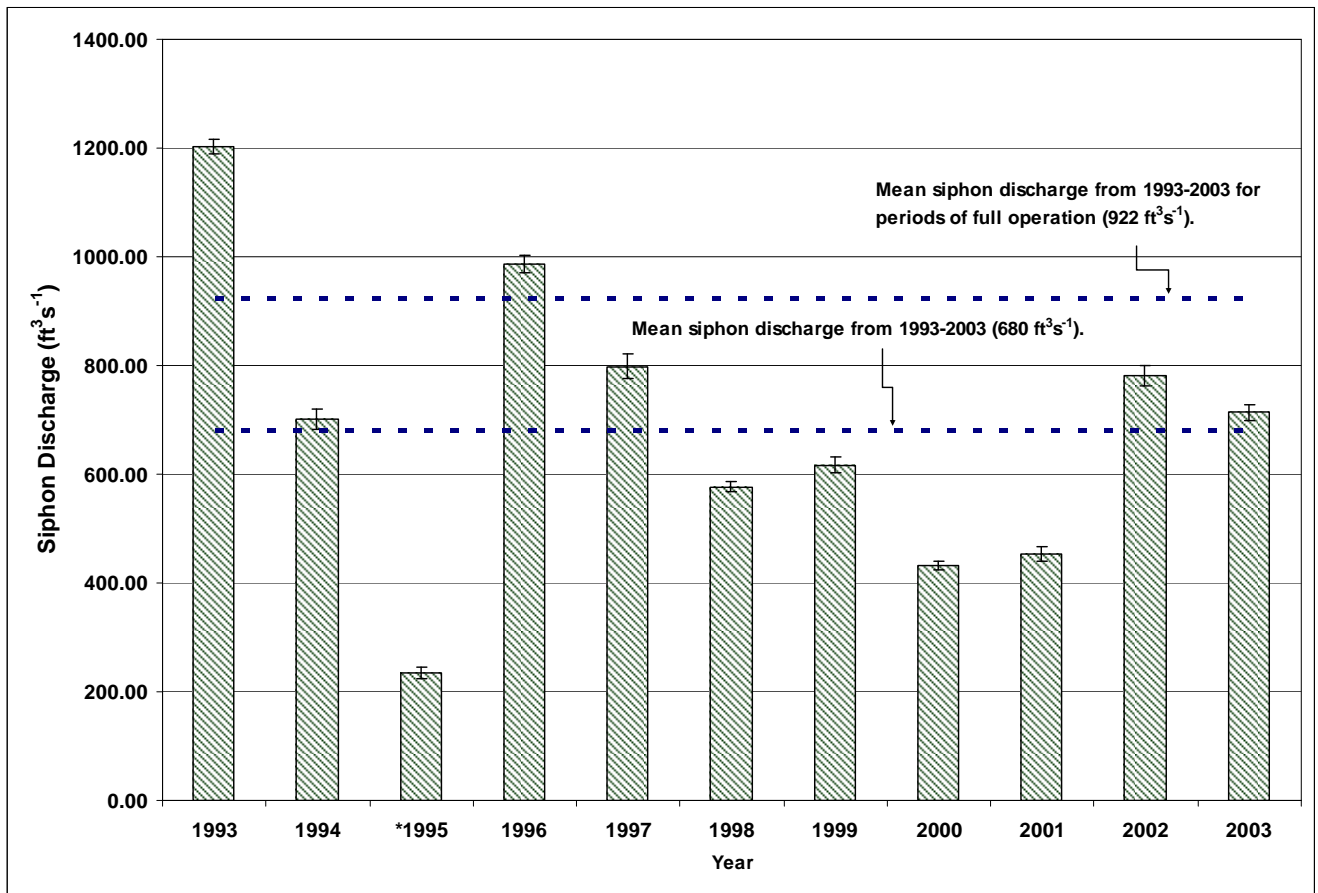
Figure 3. BA-04 yearly mean ( \pm SE) siphon discharge from 1993-2003. Dotted lines represent mean discharge during period when siphons were in full operation and the overall average for 1993-2003. Daily siphon discharge data was estimated from the Mississippi River gauge at West Pointe a la Hache LA, the immediate staff gauge in the outfall area, and the number of siphons in operation. *Siphons were not operational for 9 months during 1995.
