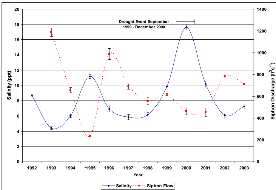
Figure 5. BA-04 West Pointe a la Hache project yearly mean ( \pm SE) salinity and siphon discharge. Salinity was measured at 17 discrete monthly hydrologic stations from 1992-2003. *Siphons were not operational for 9 months during 1995 and operated at a minimum in 2000.
