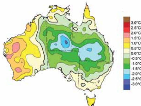
FIG. 7.52. Australian mean annual maximum temperature anomalies (base period of 1961–90) for 2010.
