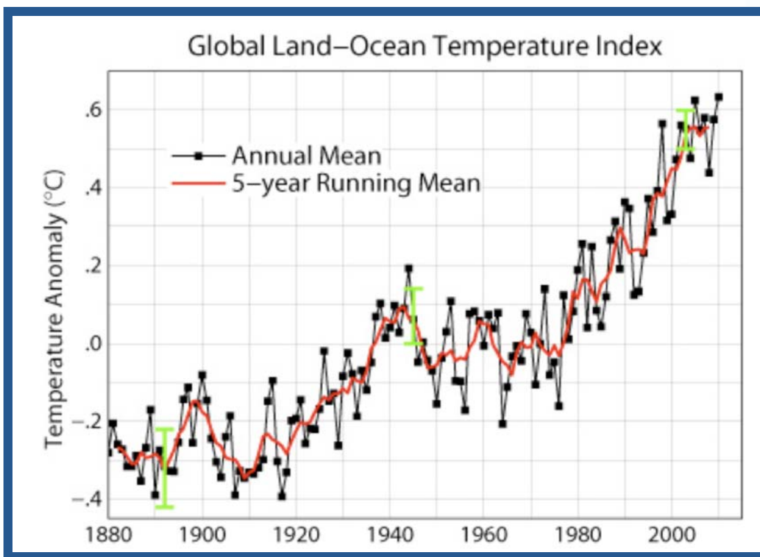
Figure 1: History of global mean surface air temperature, from the NASA Goddard Institute for Space Studies. The scale shows how much warmer or cooler the world was than the average temperature from 1951 to 1980. Recent warming is clear but with high year to year variability. The green vertical lines show data variability for the indicated time periods. Other research groups have produced similar plots. The figure is modified from Figure 1a in Hansen, J., Mki. Sato, R. Ruedy, K. Lo, D.W. Lea, and M. Medina-Elizade, 2006: Global Temperature Change. Proc. Natl. Acad. Sci. , 103, 14288-14293, doi:10.1073/pnas.0606291103.
